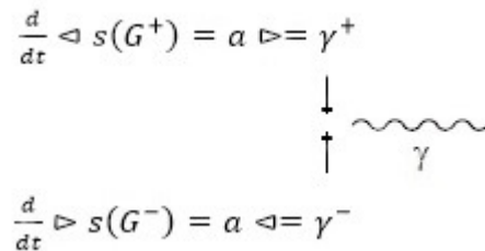
Fig2; virtual photons and real photon
